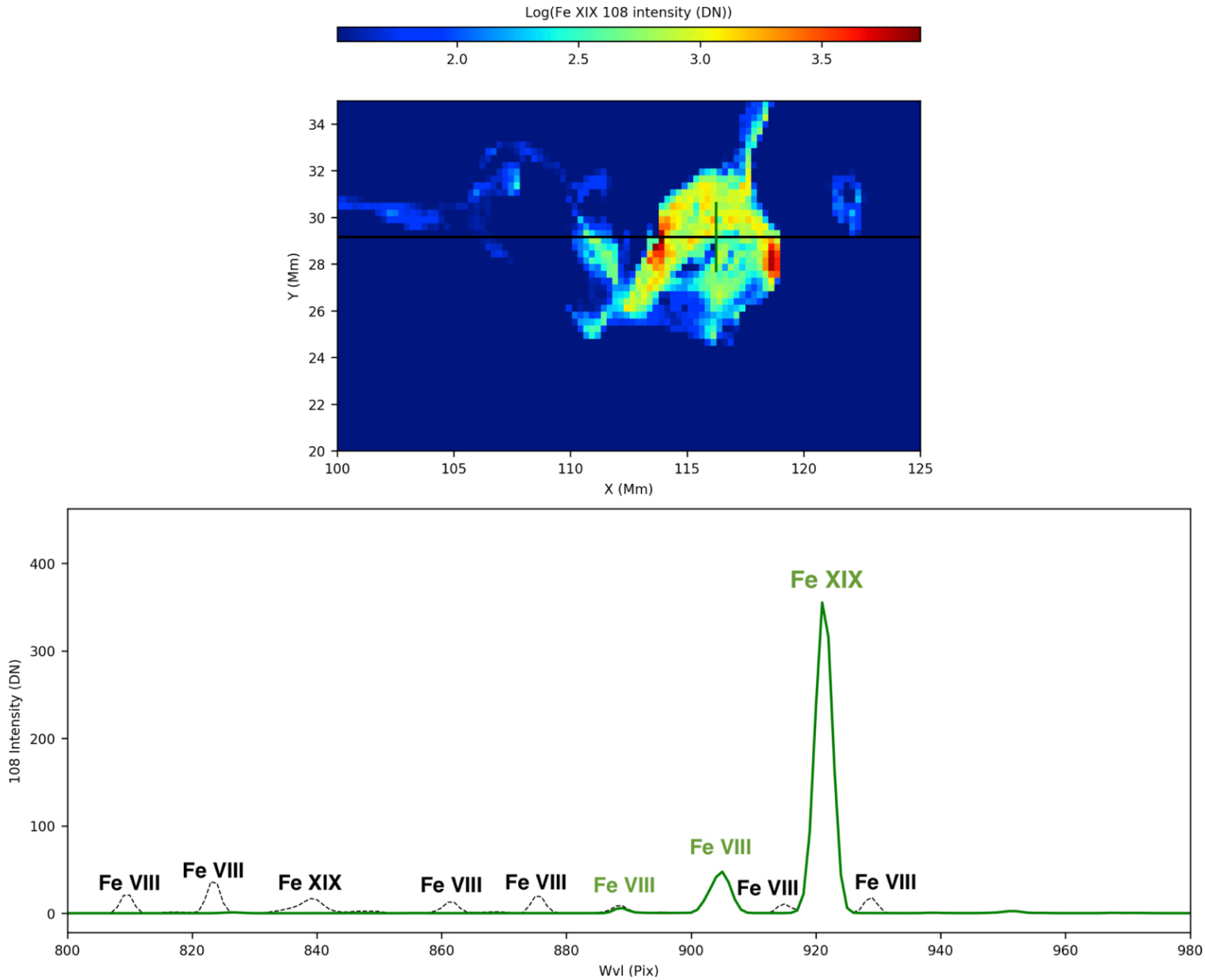
Figure 4. from The Multi-slit Approach to Coronal Spectroscopy with the Multi-slit Solar Explorer (MUSE) null 2020 APJ 888 3 doi:10.3847/1538-4357/ab5b03 https://dx.doi.org/10.3847/1538-4357/ab5b03 © 2019. The American Astronomical Society.
