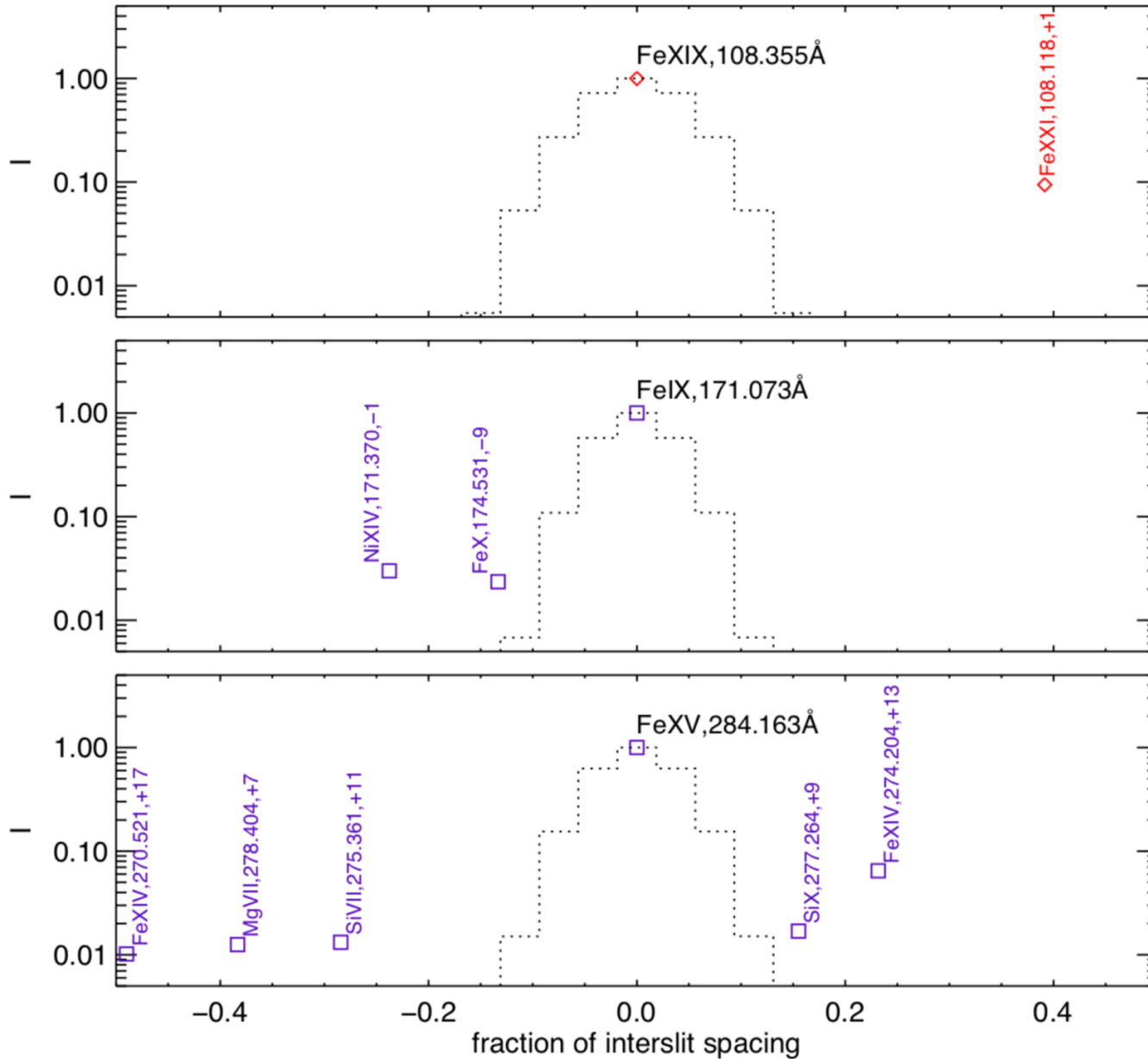
Figure 2. from The Multi-slit Approach to Coronal Spectroscopy with the Multi-slit Solar Explorer (MUSE) null 2020 APJ 888 3 doi:10.3847/1538-4357/ab5b03 https://dx.doi.org/10.3847/1538-4357/ab5b03 © 2019. The American Astronomical Society.
