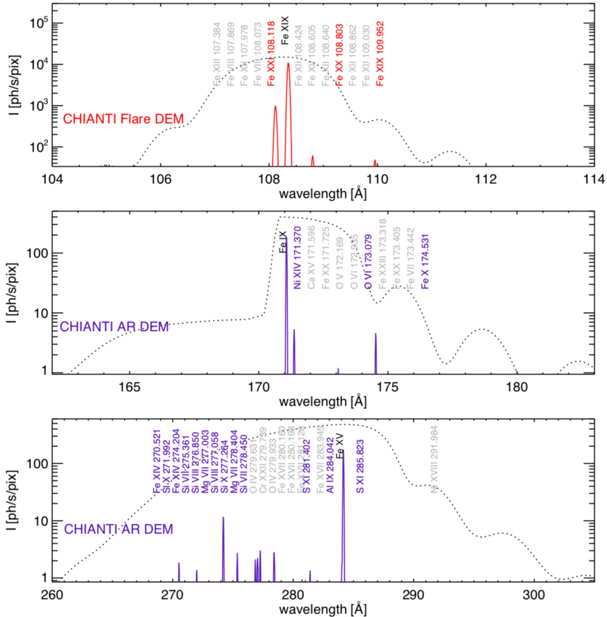
Figure 1. from The Multi-slit Approach to Coronal Spectroscopy with the Multi-slit Solar Explorer (MUSE) null 2020 APJ 888 3 doi:10.3847/1538-4357/ab5b03 https://dx.doi.org/10.3847/1538-4357/ab5b03 © 2019. The American Astronomical Society.
