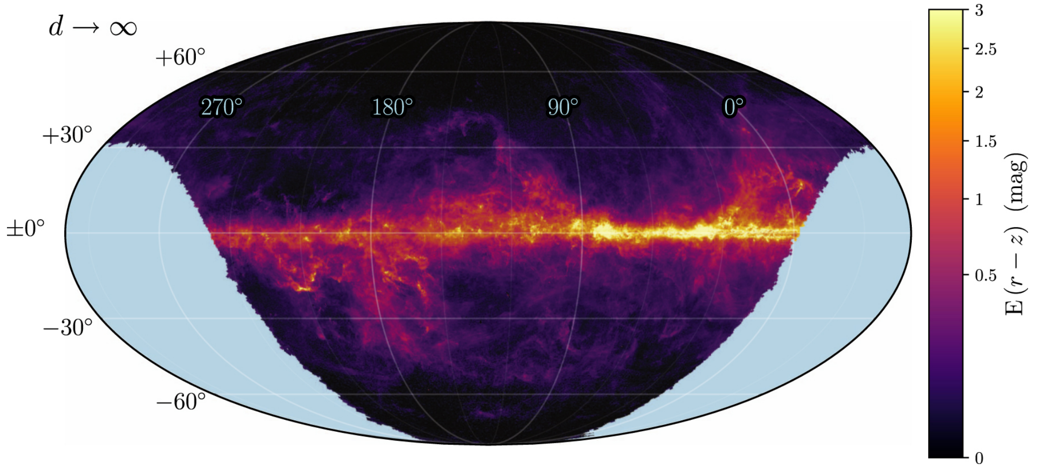
Figure 5. from A 3D Dust Map Based on Gaia, Pan-STARRS 1, and 2MASS null 2019 APJ 887 93 doi:10.3847/1538-4357/ab5362 https://dx.doi.org/10.3847/1538-4357/ab5362 © 2019. The American Astronomical Society. All rights reserved.
