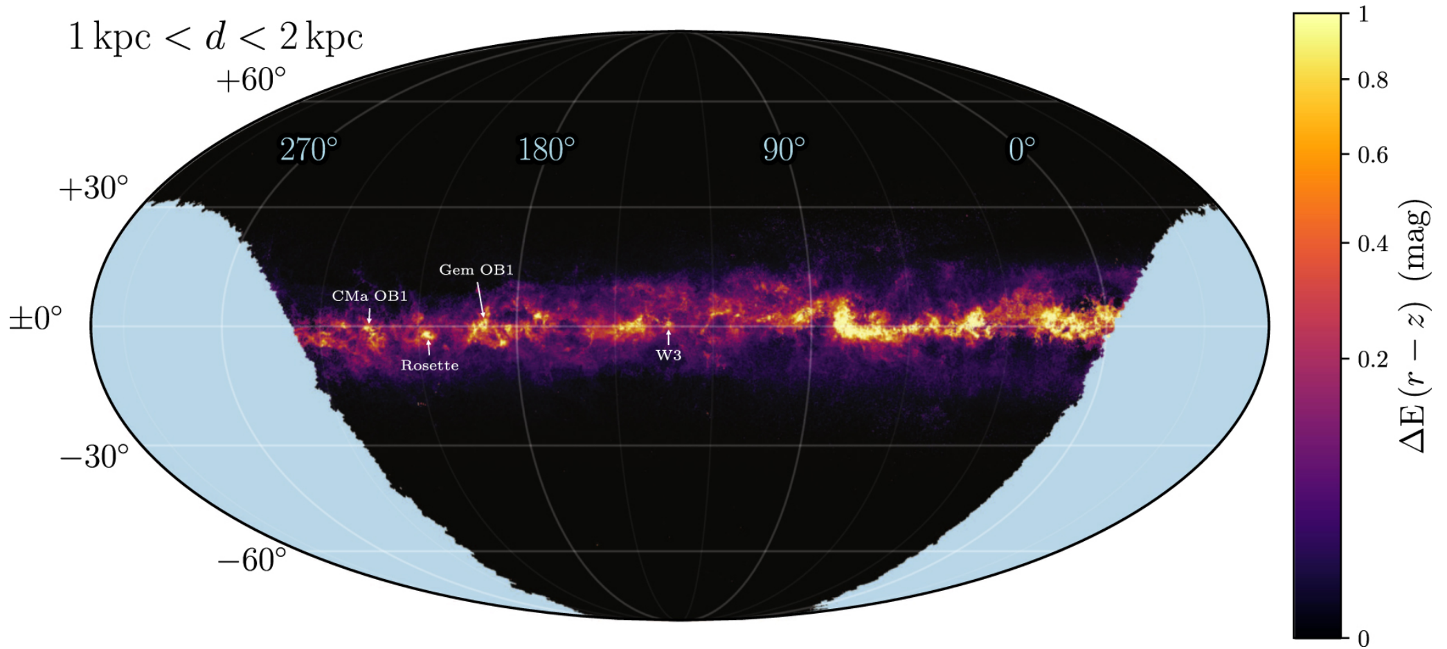
Figure 3. from A 3D Dust Map Based on Gaia, Pan-STARRS 1, and 2MASS null 2019 APJ 887 93 doi:10.3847/1538-4357/ab5362 https://dx.doi.org/10.3847/1538-4357/ab5362 © 2019. The American Astronomical Society. All rights reserved.
