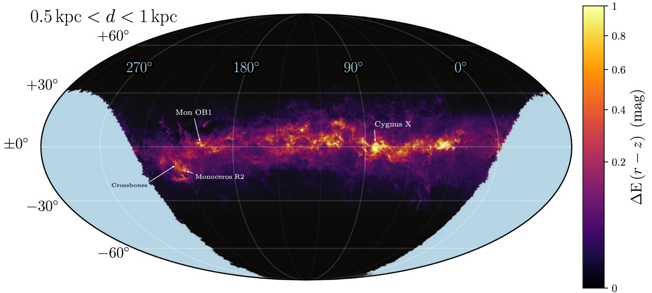
Figure 2. from A 3D Dust Map Based on Gaia, Pan-STARRS 1, and 2MASS null 2019 APJ 887 93 doi:10.3847/1538-4357/ab5362 https://dx.doi.org/10.3847/1538-4357/ab5362 © 2019. The American Astronomical Society. All rights reserved.
