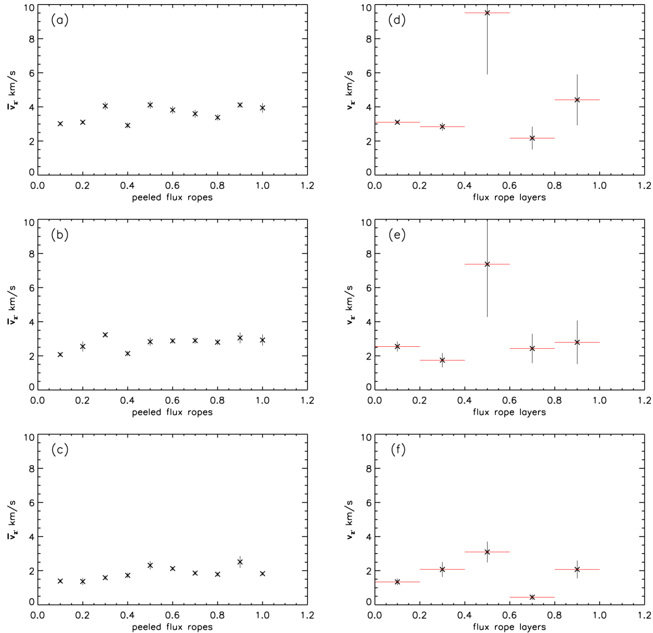
Figure 3. from The Relationship of Magnetic Twist and Plasma Motion in a Magnetic Cloud null 2019 APJ 885 122 doi:10.3847/1538-4357/ab48e5 https://dx.doi.org/10.3847/1538-4357/ab48e5 © 2019. The American Astronomical Society. All rights reserved.
