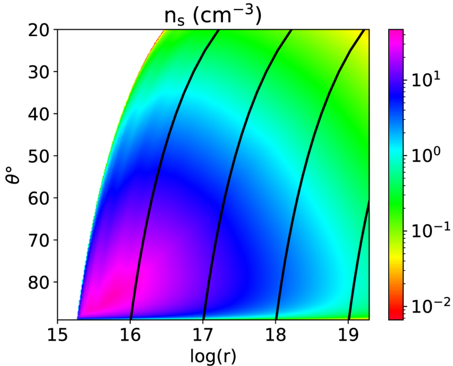
Figure 8. from Dust Formation in AGN Winds null 2019 APJ 885 126 doi:10.3847/1538-4357/ab46a9 https://dx.doi.org/10.3847/1538-4357/ab46a9 © 2019. The American Astronomical Society. All rights reserved.
