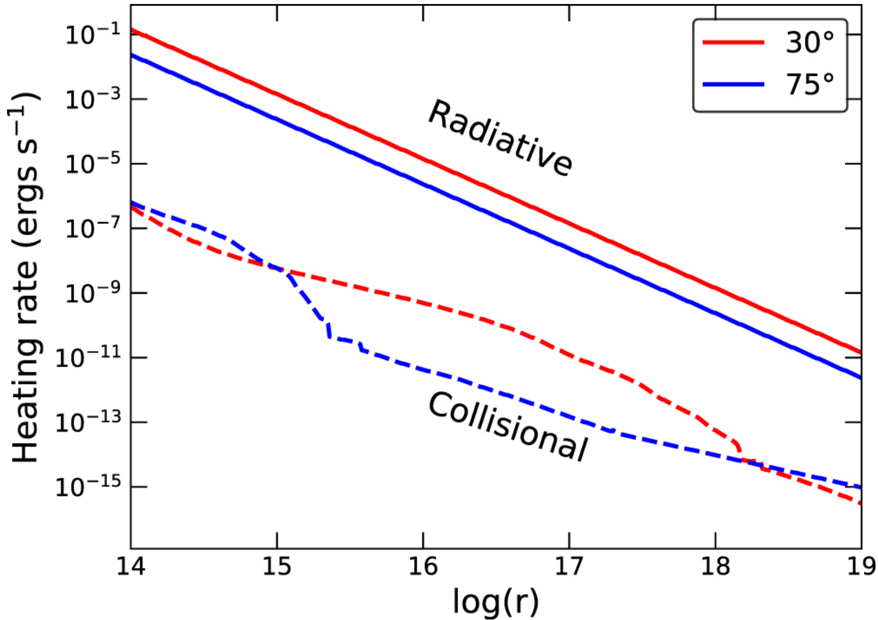
Figure 5. from Dust Formation in AGN Winds null 2019 APJ 885 126 doi:10.3847/1538-4357/ab46a9 https://dx.doi.org/10.3847/1538-4357/ab46a9 © 2019. The American Astronomical Society. All rights reserved.
