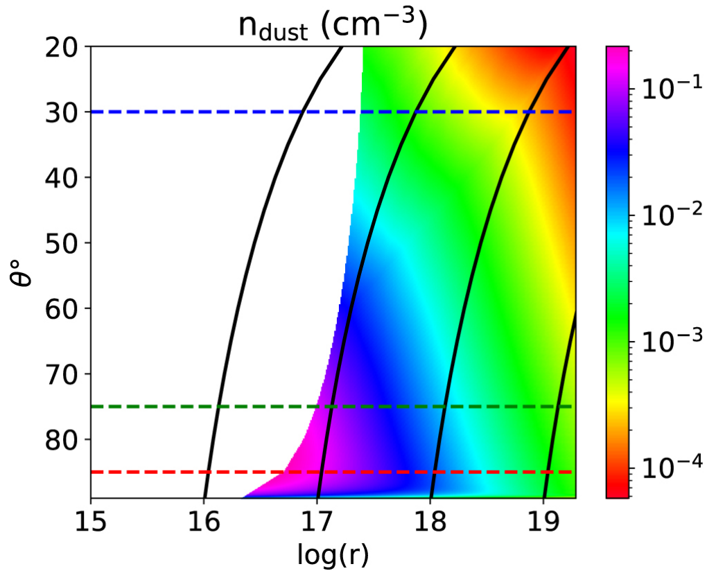
Figure 10. from Dust Formation in AGN Winds null 2019 APJ 885 126 doi:10.3847/1538-4357/ab46a9 https://dx.doi.org/10.3847/1538-4357/ab46a9 © 2019. The American Astronomical Society. All rights reserved.
