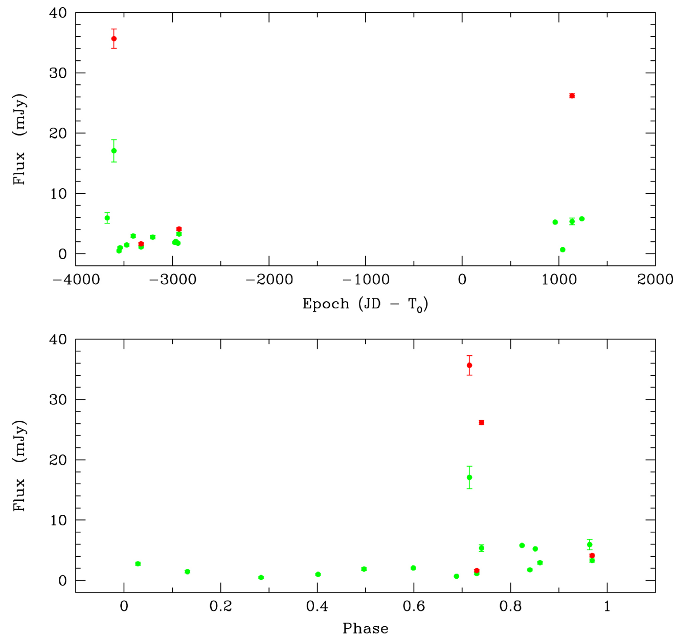
Figure 9. from Substellar Companions of the Young Weak-line TTauri Star DoAr21 null 2019 APJ 884 13 doi:10.3847/1538-4357/ab40ac https://dx.doi.org/10.3847/1538-4357/ab40ac © 2019. The American Astronomical Society. All rights reserved.
