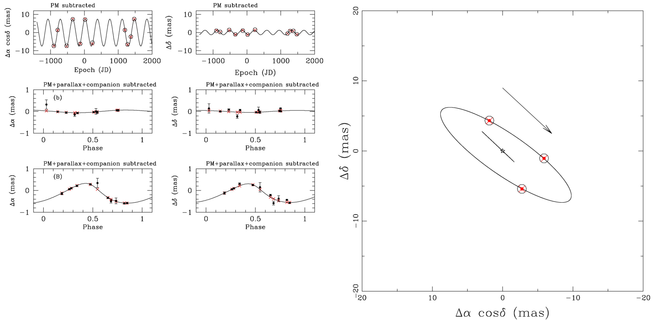
Figure 8. from Substellar Companions of the Young Weak-line TTauri Star DoAr21 null 2019 APJ 884 13 doi:10.3847/1538-4357/ab40ac https://dx.doi.org/10.3847/1538-4357/ab40ac © 2019. The American Astronomical Society. All rights reserved.
