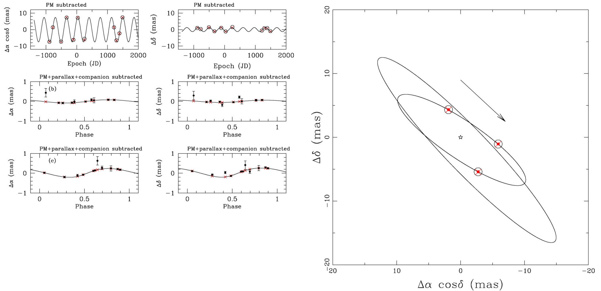
Figure 7. from Substellar Companions of the Young Weak-line TTauri Star DoAr21 null 2019 APJ 884 13 doi:10.3847/1538-4357/ab40ac https://dx.doi.org/10.3847/1538-4357/ab40ac © 2019. The American Astronomical Society. All rights reserved.
