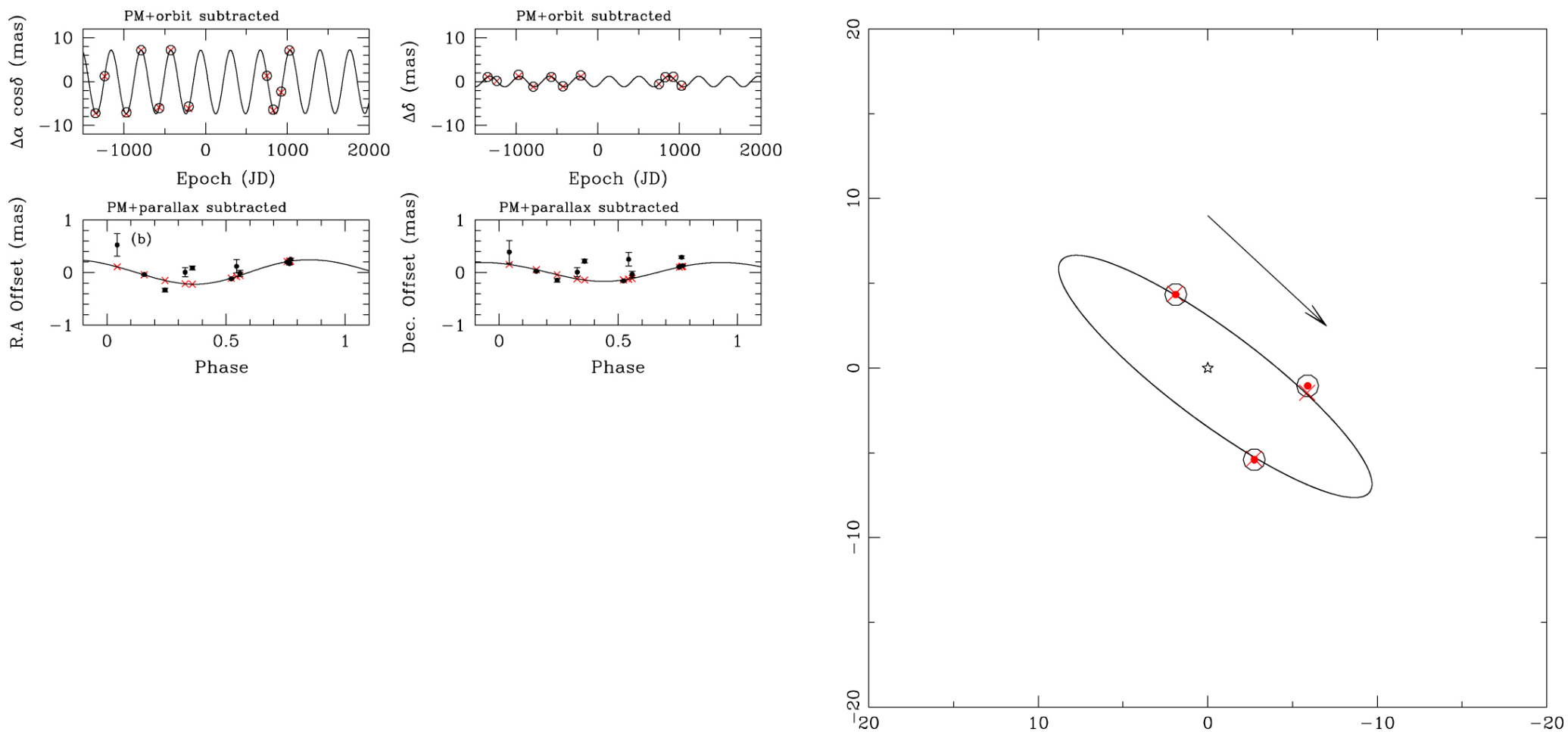
Figure 6. from Substellar Companions of the Young Weak-line TTauri Star DoAr21 null 2019 APJ 884 13 doi:10.3847/1538-4357/ab40ac https://dx.doi.org/10.3847/1538-4357/ab40ac © 2019. The American Astronomical Society. All rights reserved.
