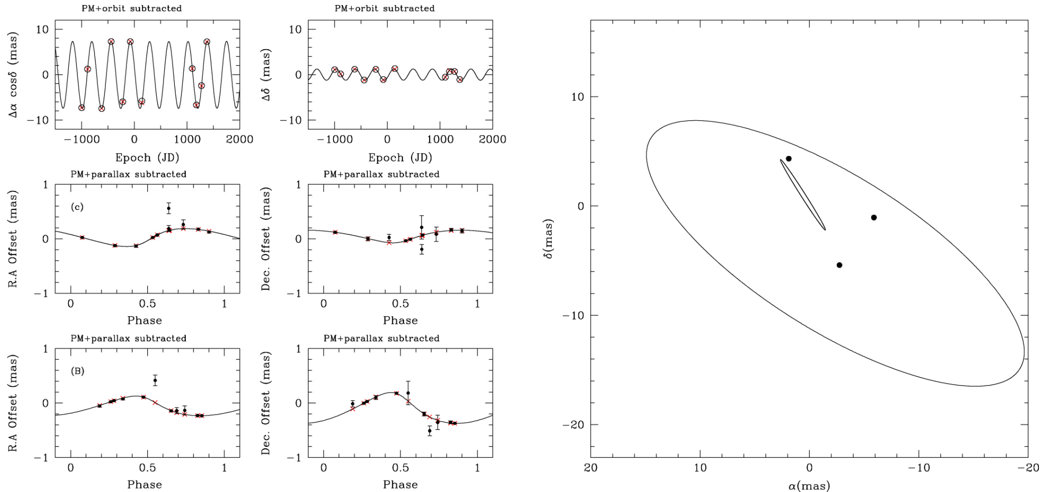
Figure 5. from Substellar Companions of the Young Weak-line TTauri Star DoAr21 null 2019 APJ 884 13 doi:10.3847/1538-4357/ab40ac https://dx.doi.org/10.3847/1538-4357/ab40ac © 2019. The American Astronomical Society. All rights reserved.
