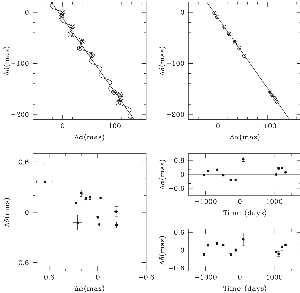
Figure 3. from Substellar Companions of the Young Weak-line TTauri Star DoAr21 null 2019 APJ 884 13 doi:10.3847/1538-4357/ab40ac https://dx.doi.org/10.3847/1538-4357/ab40ac © 2019. The American Astronomical Society. All rights reserved.
