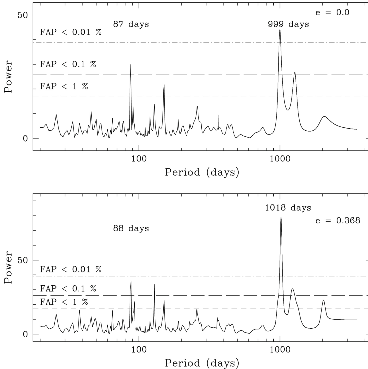
Figure 2. from Substellar Companions of the Young Weak-line TTauri Star DoAr21 null 2019 APJ 884 13 doi:10.3847/1538-4357/ab40ac https://dx.doi.org/10.3847/1538-4357/ab40ac © 2019. The American Astronomical Society. All rights reserved.
