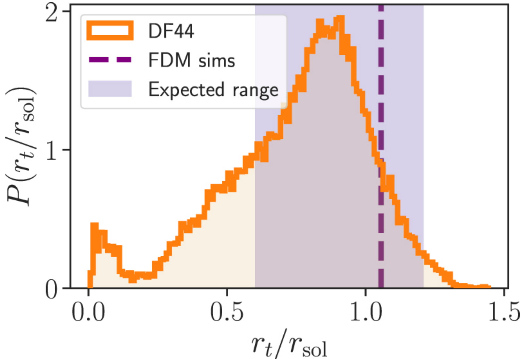
Figure 9. from Spatially Resolved Stellar Kinematics of the Ultra-diffuse Galaxy Dragonfly 44. II. Constraints on Fuzzy Dark Matter null 2019 APJ 885 155 doi:10.3847/1538-4357/ab3eb9 https://dx.doi.org/10.3847/1538-4357/ab3eb9 © 2019. The American Astronomical Society. All rights reserved.
