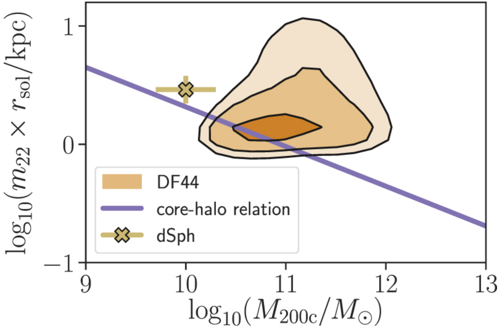
Figure 8. from Spatially Resolved Stellar Kinematics of the Ultra-diffuse Galaxy Dragonfly 44. II. Constraints on Fuzzy Dark Matter null 2019 APJ 885 155 doi:10.3847/1538-4357/ab3eb9 https://dx.doi.org/10.3847/1538-4357/ab3eb9 © 2019. The American Astronomical Society. All rights reserved.
