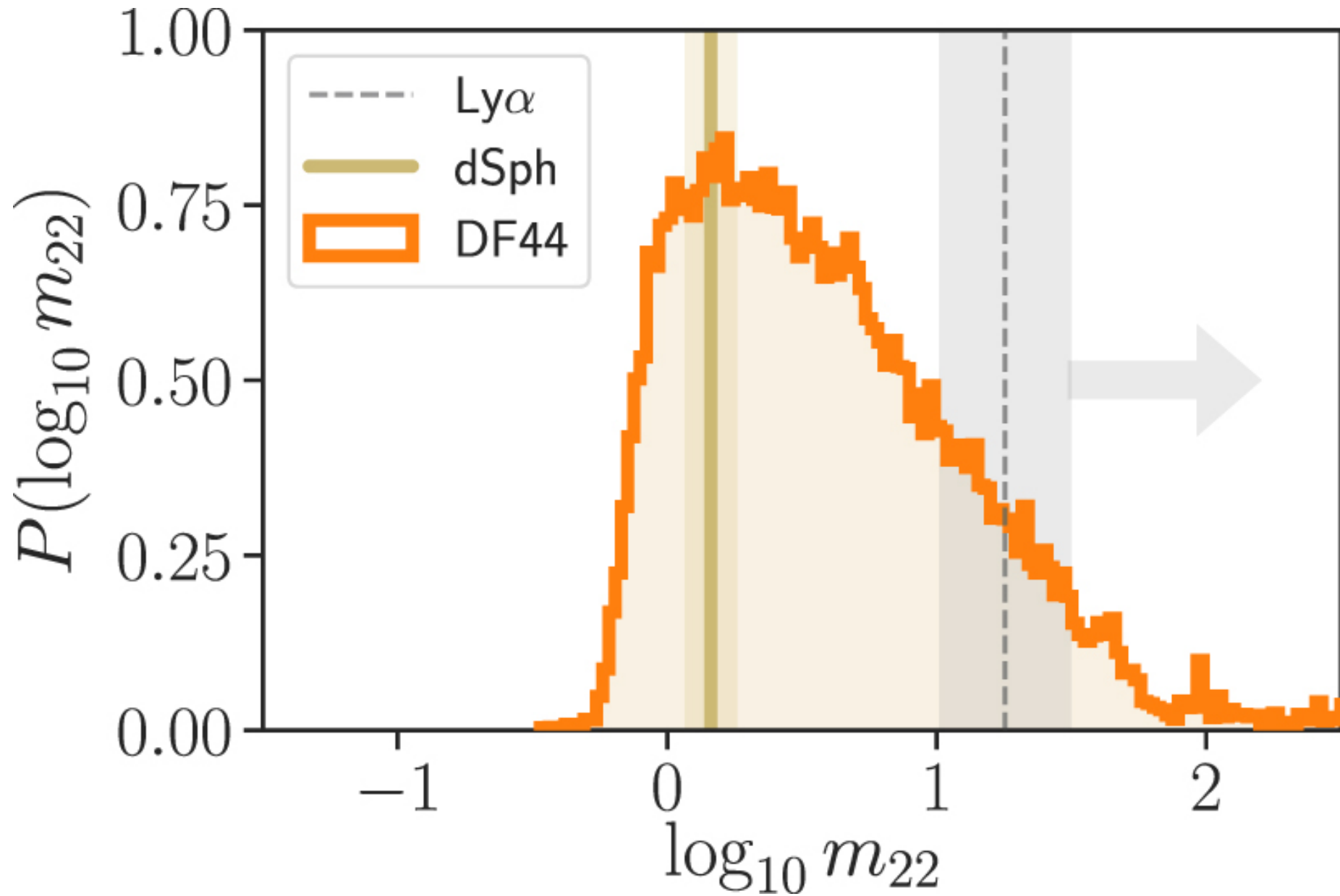
Figure 7. from Spatially Resolved Stellar Kinematics of the Ultra-diffuse Galaxy Dragonfly 44. II. Constraints on Fuzzy Dark Matter null 2019 APJ 885 155 doi:10.3847/1538-4357/ab3eb9 https://dx.doi.org/10.3847/1538-4357/ab3eb9 © 2019. The American Astronomical Society. All rights reserved.
