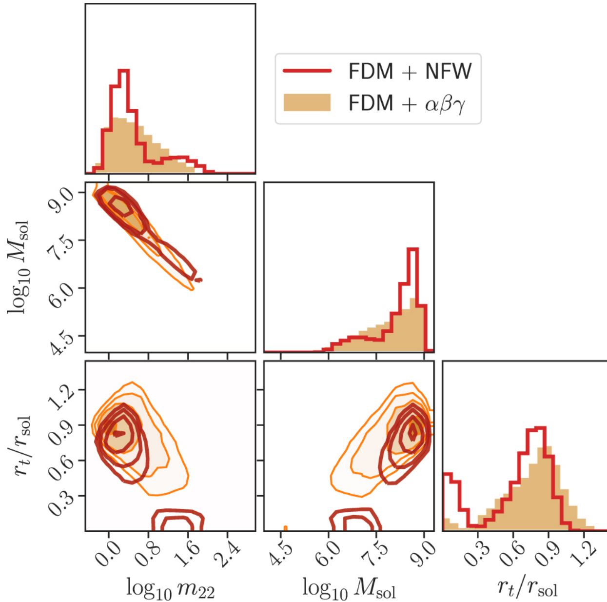
Figure 6. from Spatially Resolved Stellar Kinematics of the Ultra-diffuse Galaxy Dragonfly 44. II. Constraints on Fuzzy Dark Matter null 2019 APJ 885 155 doi:10.3847/1538-4357/ab3eb9 https://dx.doi.org/10.3847/1538-4357/ab3eb9 © 2019. The American Astronomical Society. All rights reserved.
