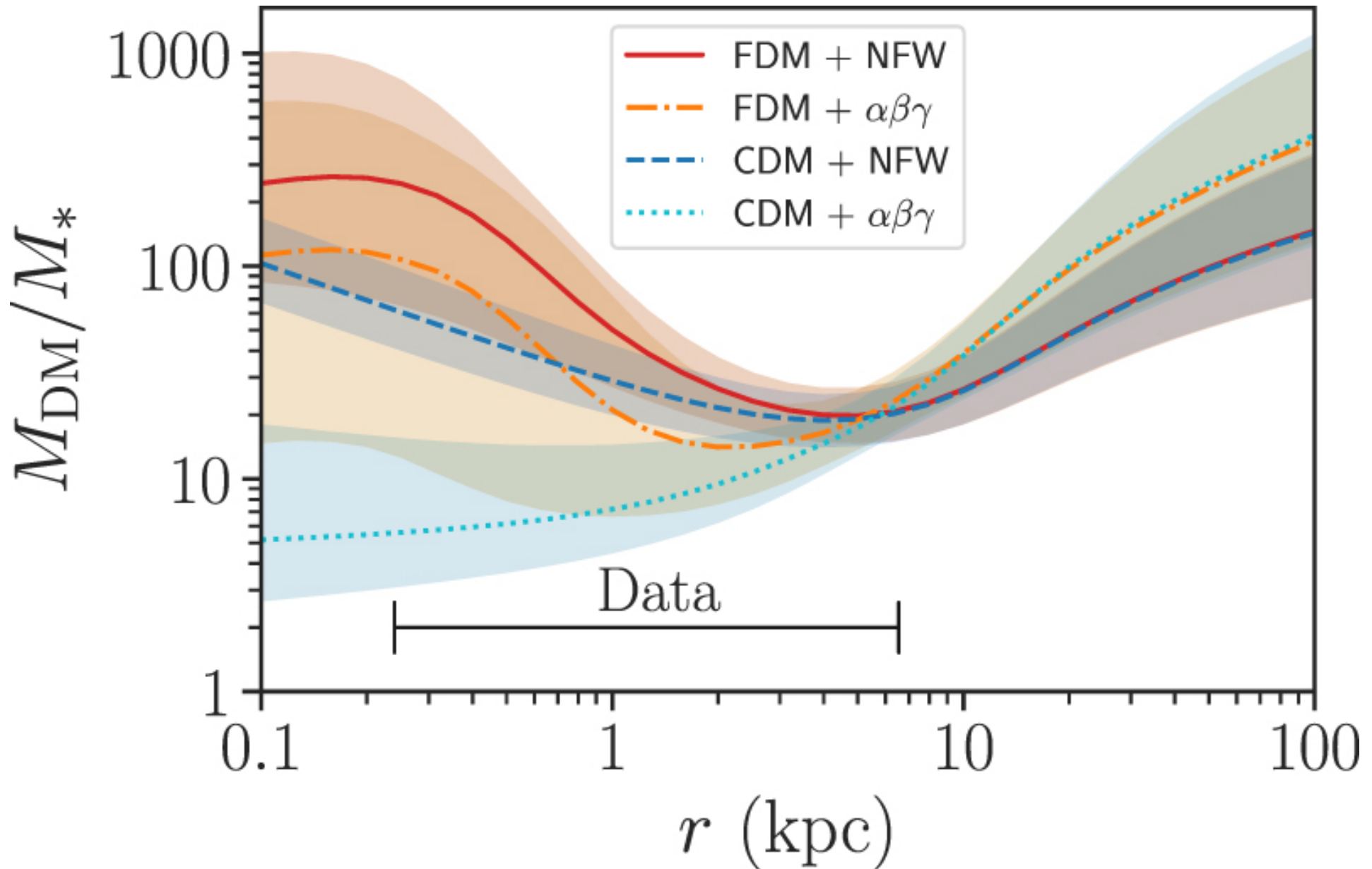
Figure 5. from Spatially Resolved Stellar Kinematics of the Ultra-diffuse Galaxy Dragonfly 44. II. Constraints on Fuzzy Dark Matter null 2019 APJ 885 155 doi:10.3847/1538-4357/ab3eb9 https://dx.doi.org/10.3847/1538-4357/ab3eb9 © 2019. The American Astronomical Society. All rights reserved.
