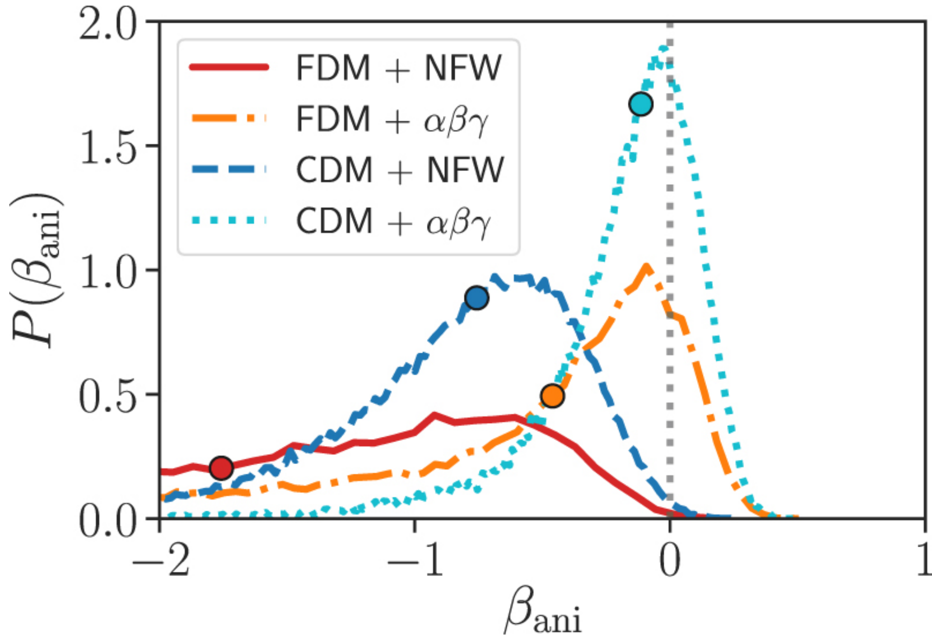
Figure 4. from Spatially Resolved Stellar Kinematics of the Ultra-diffuse Galaxy Dragonfly 44. II. Constraints on Fuzzy Dark Matter null 2019 APJ 885 155 doi:10.3847/1538-4357/ab3eb9 https://dx.doi.org/10.3847/1538-4357/ab3eb9 © 2019. The American Astronomical Society. All rights reserved.
