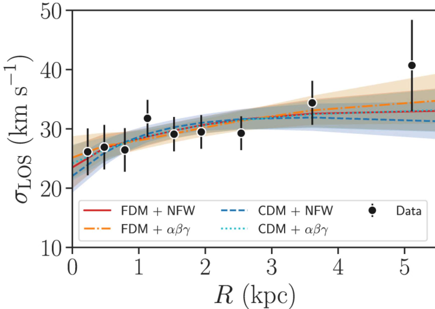
Figure 2. from Spatially Resolved Stellar Kinematics of the Ultra-diffuse Galaxy Dragonfly 44. II. Constraints on Fuzzy Dark Matter null 2019 APJ 885 155 doi:10.3847/1538-4357/ab3eb9 https://dx.doi.org/10.3847/1538-4357/ab3eb9 © 2019. The American Astronomical Society. All rights reserved.
