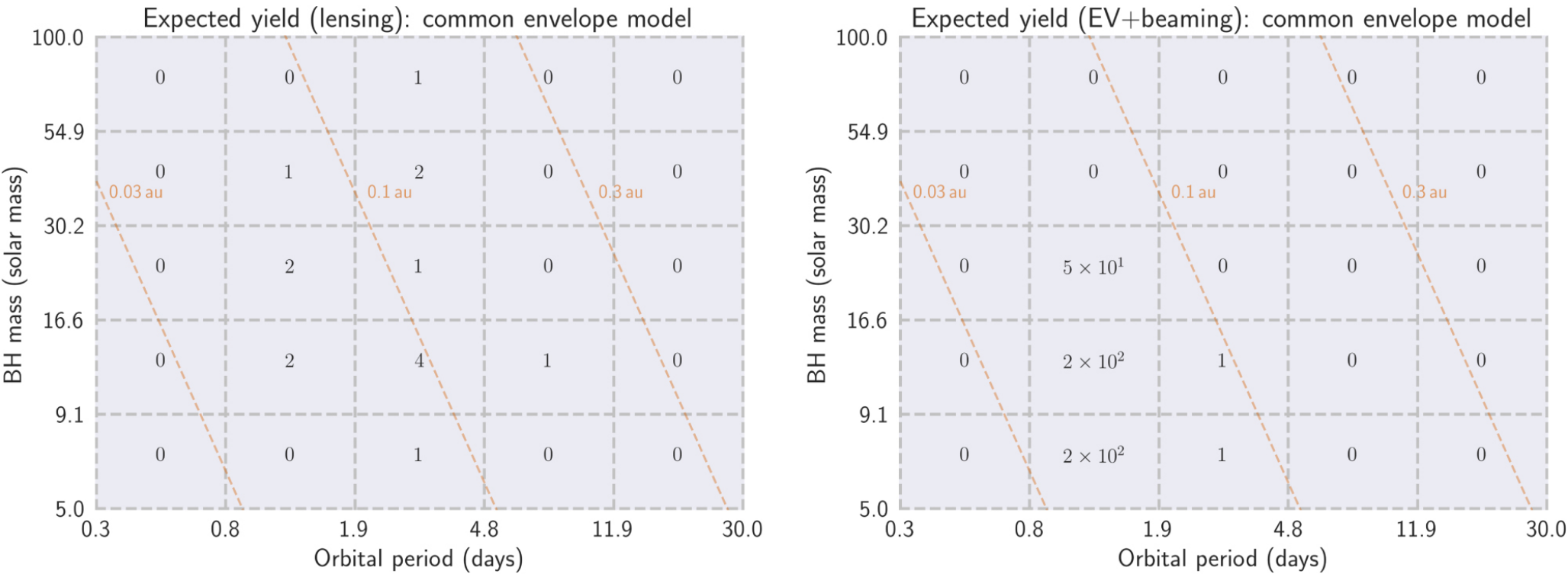
Figure 6. from Prospects of Finding Detached Black Hole–Star Binaries with TESS null 2019 APJ 883 169 doi:10.3847/1538-4357/ab3a4f https://dx.doi.org/10.3847/1538-4357/ab3a4f © 2019. The American Astronomical Society. All rights reserved.
