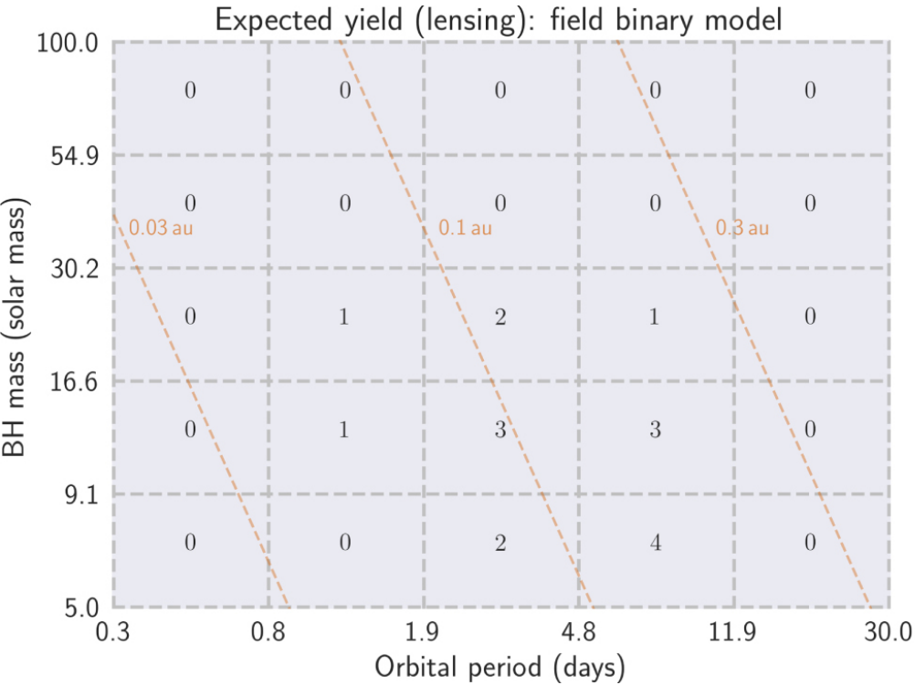
Figure 5. from Prospects of Finding Detached Black Hole–Star Binaries with TESS null 2019 APJ 883 169 doi:10.3847/1538-4357/ab3a4f https://dx.doi.org/10.3847/1538-4357/ab3a4f © 2019. The American Astronomical Society. All rights reserved.
