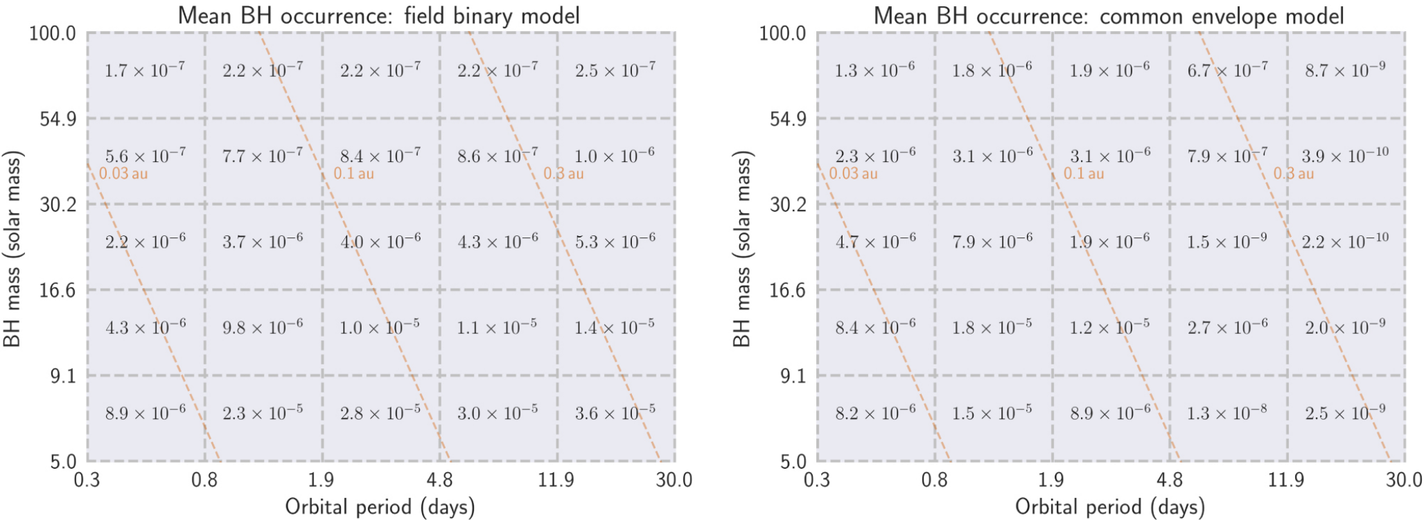
Figure 4. from Prospects of Finding Detached Black Hole–Star Binaries with TESS null 2019 APJ 883 169 doi:10.3847/1538-4357/ab3a4f https://dx.doi.org/10.3847/1538-4357/ab3a4f © 2019. The American Astronomical Society. All rights reserved.
