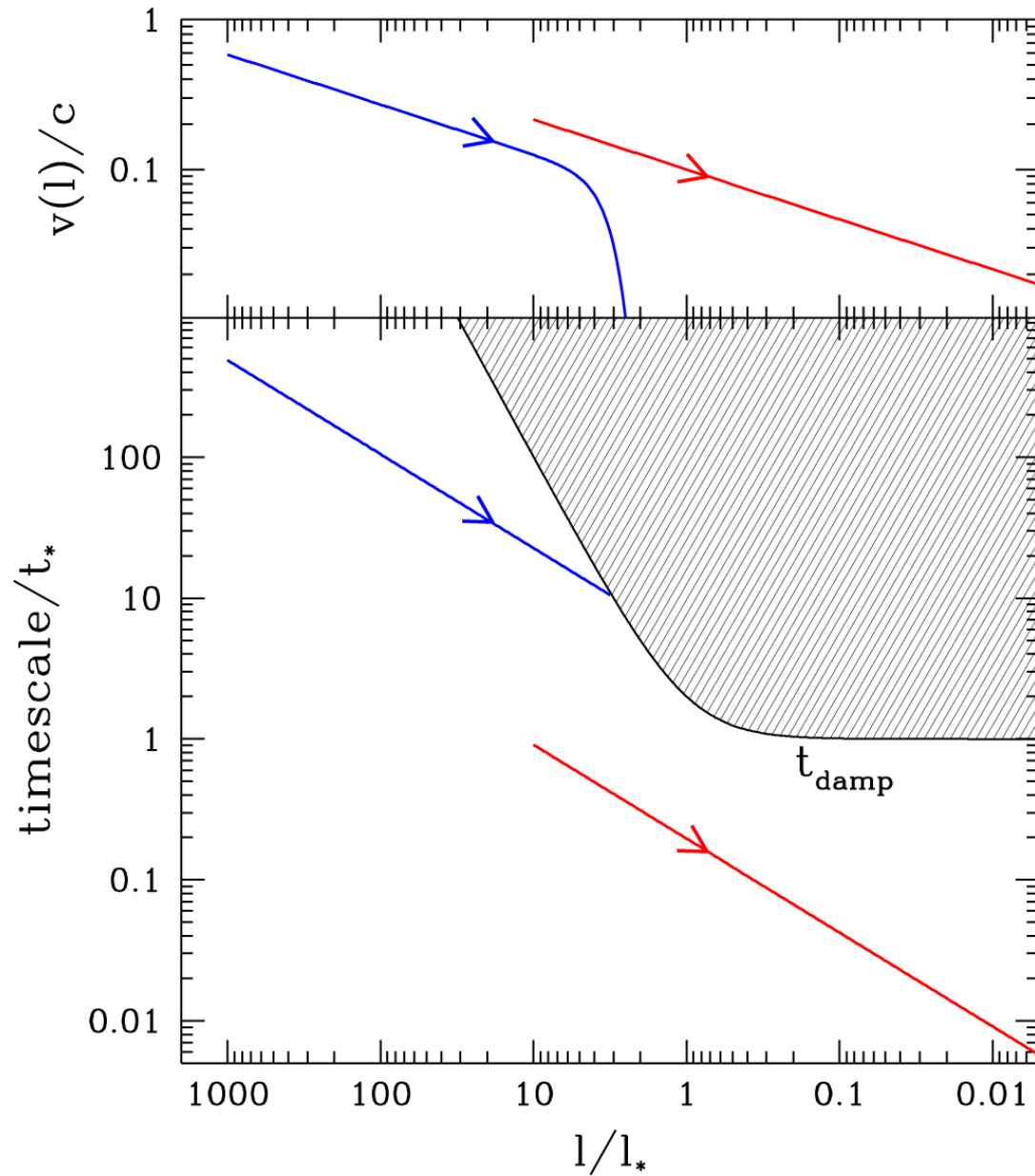
Figure 2. from Subphotospheric Turbulence as a Heating Mechanism in Gamma-Ray Bursts null 2019 APJ 885 30 doi:10.3847/1538-4357/ab364b https://dx.doi.org/10.3847/1538-4357/ab364b © 2019. The American Astronomical Society. All rights reserved.
