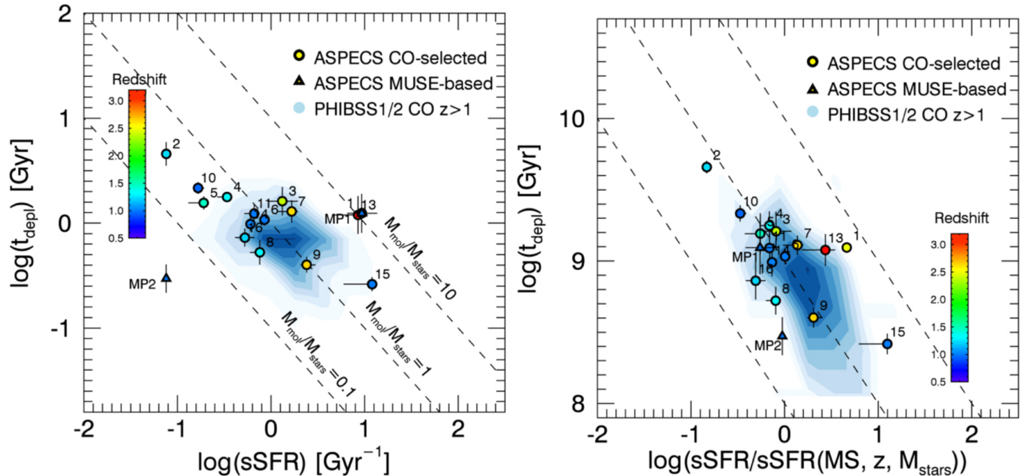
Figure 9. from The ALMA Spectroscopic Survey in the Hubble Ultra Deep Field: Evolution of the Molecular Gas in CO-selected Galaxies null 2019 APJ 882 136 doi:10.3847/1538-4357/ab30df https://dx.doi.org/10.3847/1538-4357/ab30df © 2019. The American Astronomical Society. All rights reserved.
