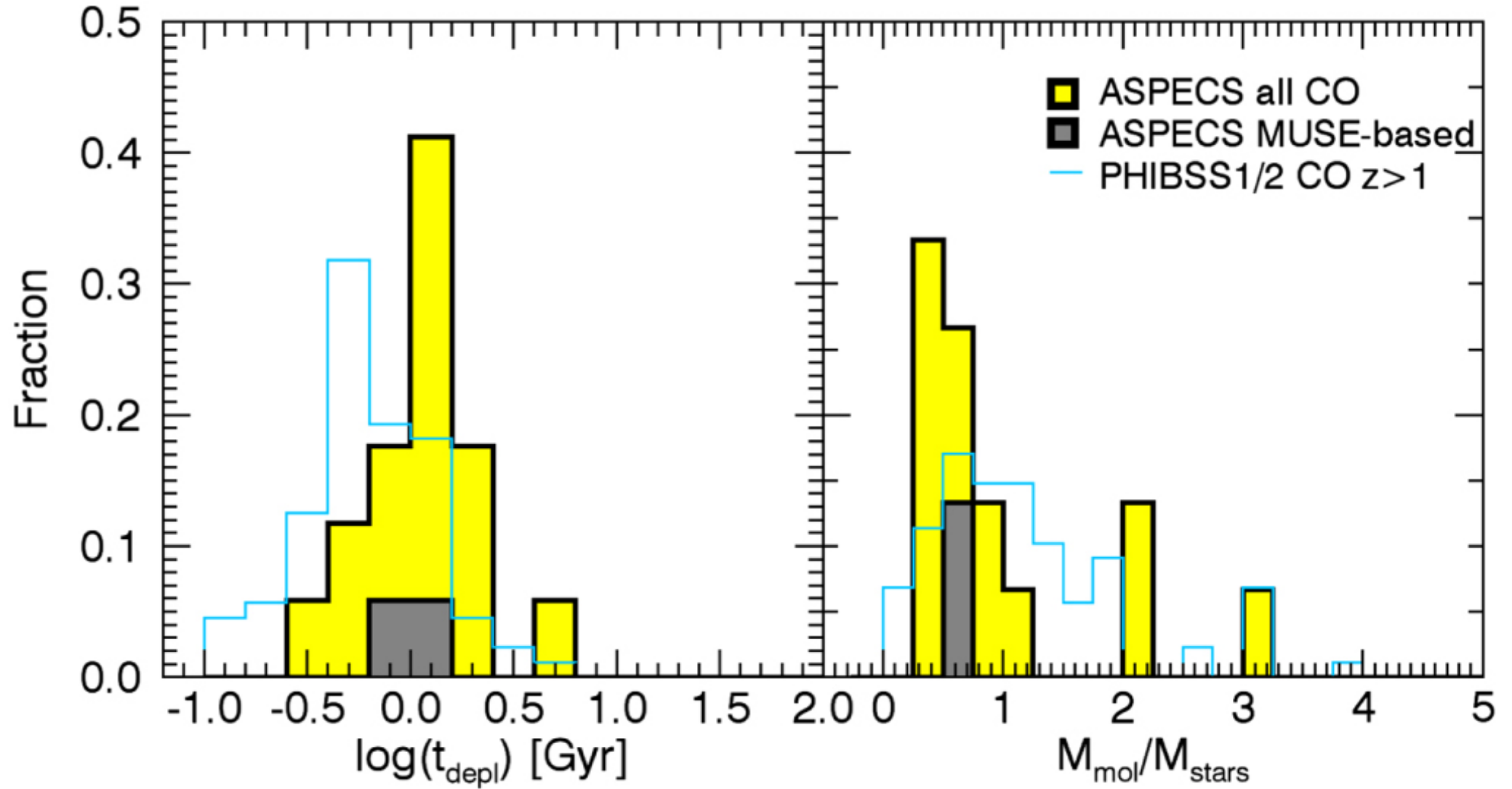
Figure 8. from The ALMA Spectroscopic Survey in the Hubble Ultra Deep Field: Evolution of the Molecular Gas in CO-selected Galaxies null 2019 APJ 882 136 doi:10.3847/1538-4357/ab30df https://dx.doi.org/10.3847/1538-4357/ab30df © 2019. The American Astronomical Society. All rights reserved.
