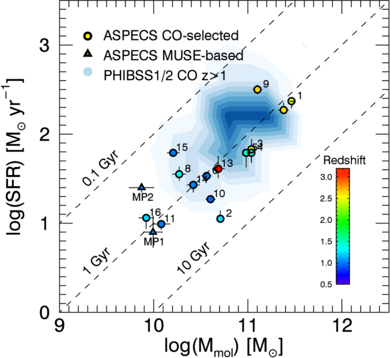
Figure 7. from The ALMA Spectroscopic Survey in the Hubble Ultra Deep Field: Evolution of the Molecular Gas in CO-selected Galaxies null 2019 APJ 882 136 doi:10.3847/1538-4357/ab30df https://dx.doi.org/10.3847/1538-4357/ab30df © 2019. The American Astronomical Society. All rights reserved.
