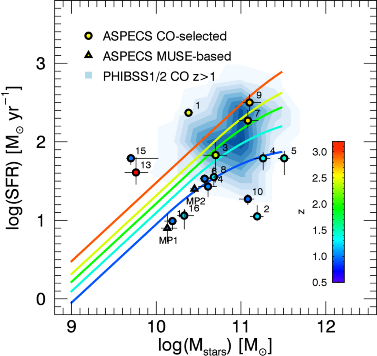
Figure 5. from The ALMA Spectroscopic Survey in the Hubble Ultra Deep Field: Evolution of the Molecular Gas in CO-selected Galaxies null 2019 APJ 882 136 doi:10.3847/1538-4357/ab30df https://dx.doi.org/10.3847/1538-4357/ab30df © 2019. The American Astronomical Society. All rights reserved.
