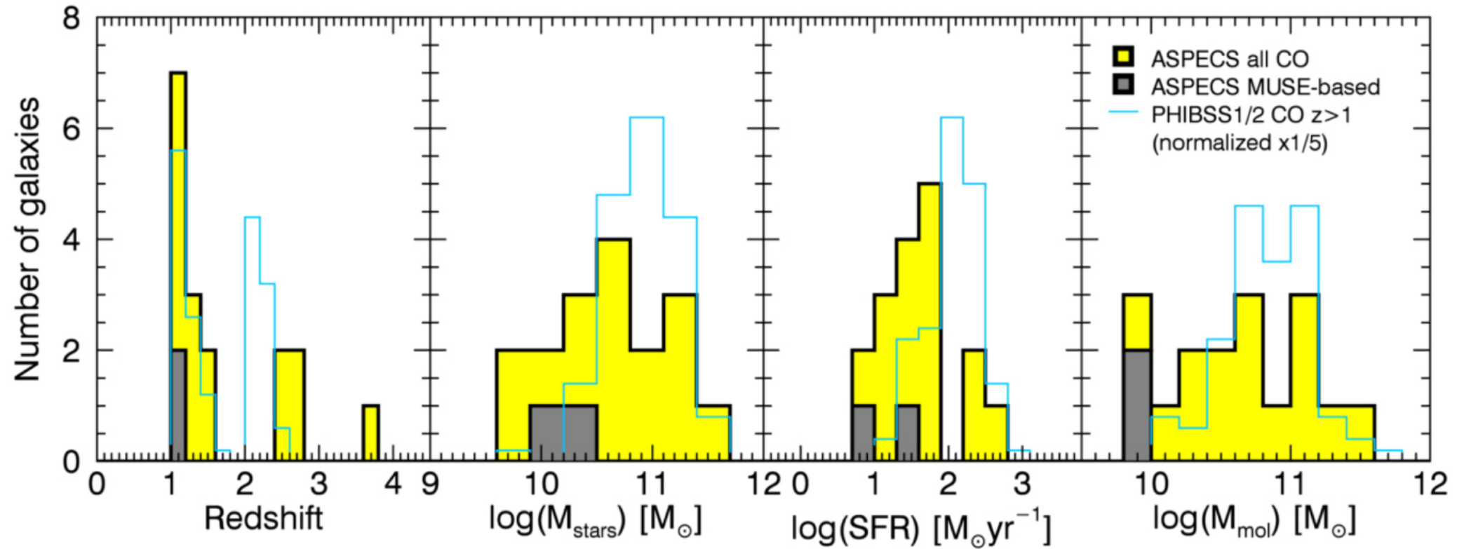
Figure 4. from The ALMA Spectroscopic Survey in the Hubble Ultra Deep Field: Evolution of the Molecular Gas in CO-selected Galaxies null 2019 APJ 882 136 doi:10.3847/1538-4357/ab30df https://dx.doi.org/10.3847/1538-4357/ab30df © 2019. The American Astronomical Society. All rights reserved.
