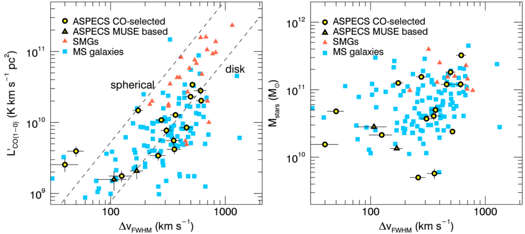
Figure 3. from The ALMA Spectroscopic Survey in the Hubble Ultra Deep Field: Evolution of the Molecular Gas in CO-selected Galaxies null 2019 APJ 882 136 doi:10.3847/1538-4357/ab30df https://dx.doi.org/10.3847/1538-4357/ab30df © 2019. The American Astronomical Society. All rights reserved.
