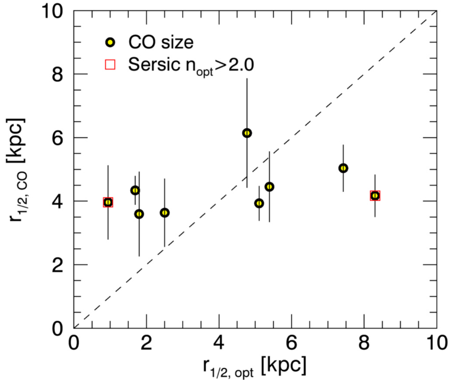
Figure 13. from The ALMA Spectroscopic Survey in the Hubble Ultra Deep Field: Evolution of the Molecular Gas in CO-selected Galaxies null 2019 APJ 882 136 doi:10.3847/1538-4357/ab30df https://dx.doi.org/10.3847/1538-4357/ab30df © 2019. The American Astronomical Society. All rights reserved.
