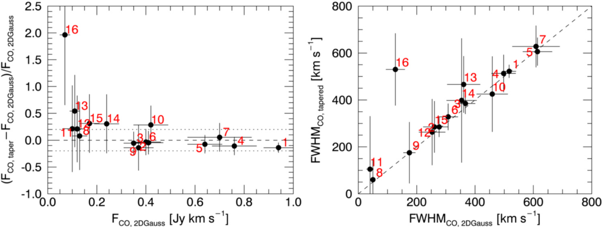
Figure 12. from The ALMA Spectroscopic Survey in the Hubble Ultra Deep Field: Evolution of the Molecular Gas in CO-selected Galaxies null 2019 APJ 882 136 doi:10.3847/1538-4357/ab30df https://dx.doi.org/10.3847/1538-4357/ab30df © 2019. The American Astronomical Society. All rights reserved.
