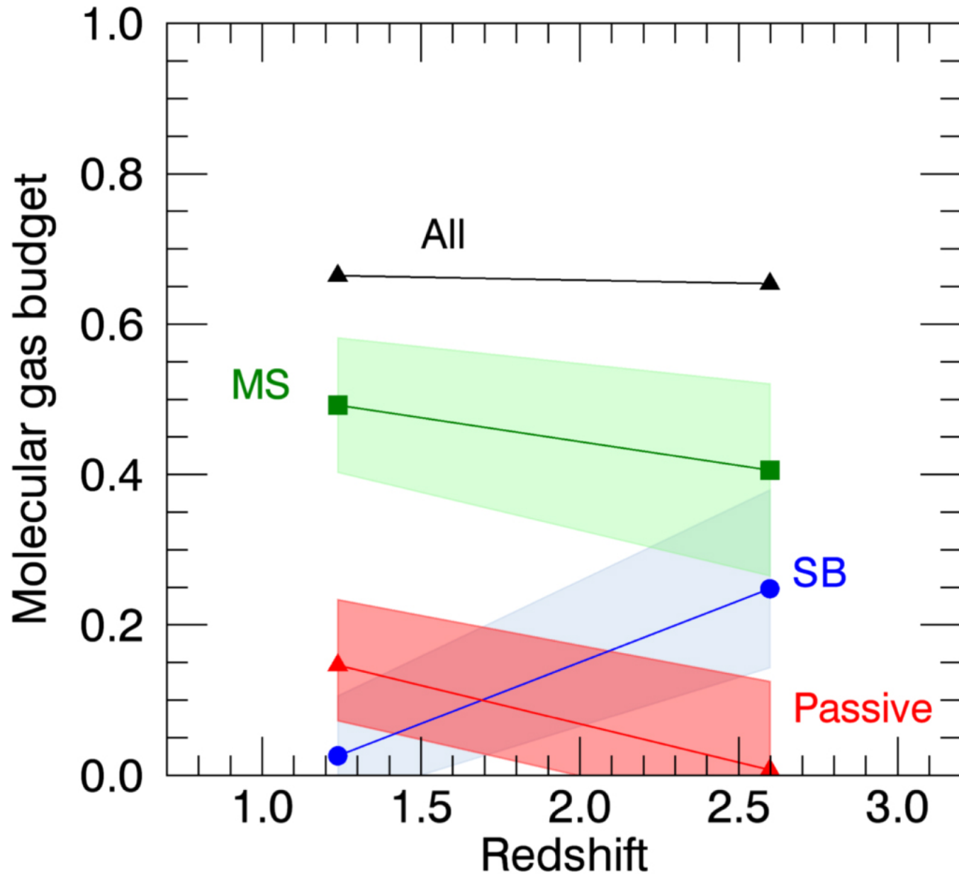
Figure 11. from The ALMA Spectroscopic Survey in the Hubble Ultra Deep Field: Evolution of the Molecular Gas in CO-selected Galaxies null 2019 APJ 882 136 doi:10.3847/1538-4357/ab30df https://dx.doi.org/10.3847/1538-4357/ab30df © 2019. The American Astronomical Society. All rights reserved.
