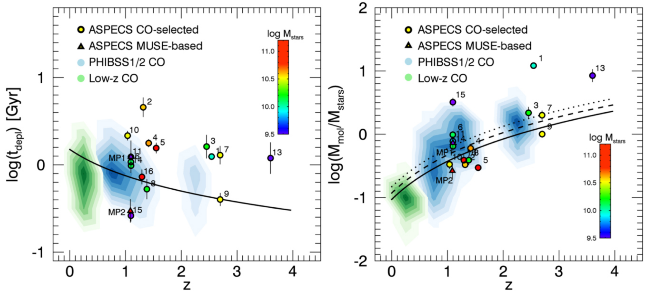
Figure 10. from The ALMA Spectroscopic Survey in the Hubble Ultra Deep Field: Evolution of the Molecular Gas in CO-selected Galaxies null 2019 APJ 882 136 doi:10.3847/1538-4357/ab30df https://dx.doi.org/10.3847/1538-4357/ab30df © 2019. The American Astronomical Society. All rights reserved.
