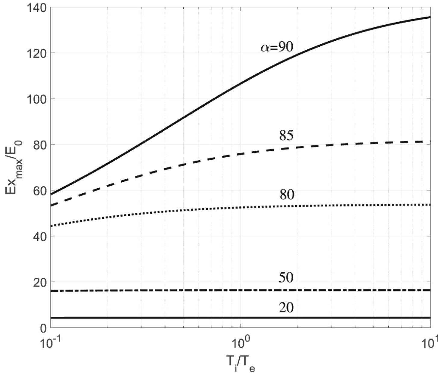
Figure 6. from Resonant Mode Conversion of Alfvén Waves to Kinetic Alfvén Waves in an Inhomogeneous Plasma null 2019 APJ 881 61 doi:10.3847/1538-4357/ab2bf1 https://dx.doi.org/10.3847/1538-4357/ab2bf1 © 2019. The American Astronomical Society. All rights reserved.
