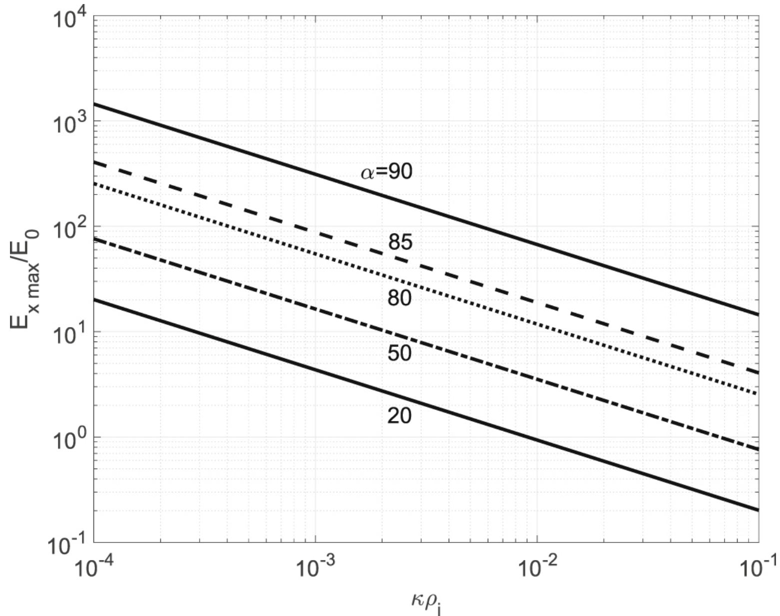
Figure 5. from Resonant Mode Conversion of Alfvén Waves to Kinetic Alfvén Waves in an Inhomogeneous Plasma null 2019 APJ 881 61 doi:10.3847/1538-4357/ab2bf1 https://dx.doi.org/10.3847/1538-4357/ab2bf1 © 2019. The American Astronomical Society. All rights reserved.
