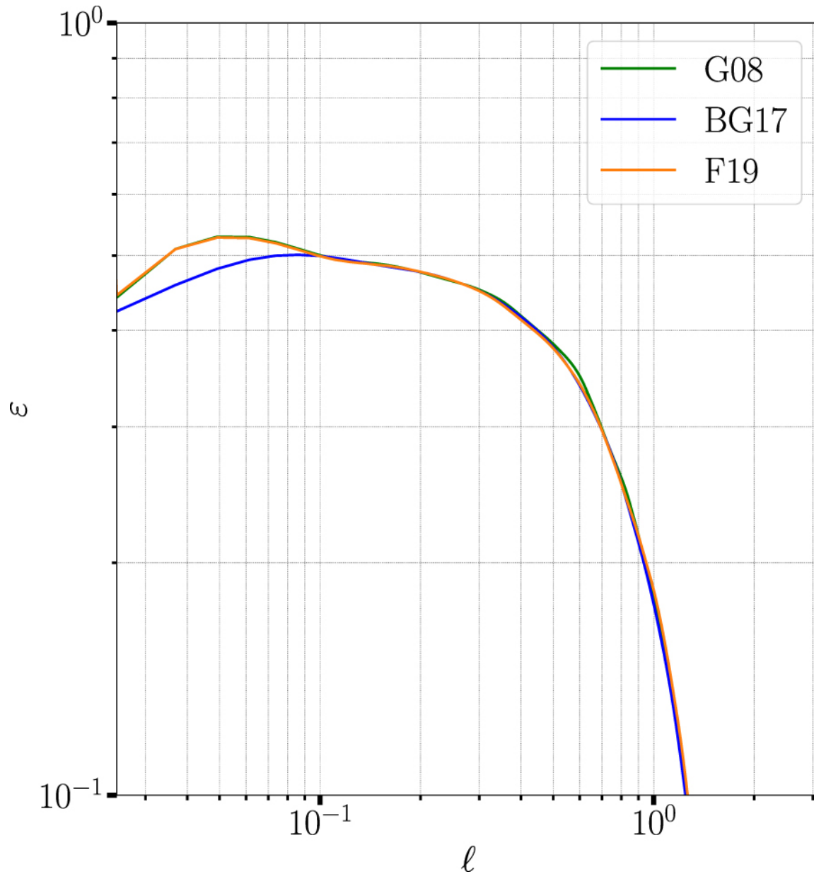
Figure 2. from On Exact Laws in Incompressible Hall Magnetohydrodynamic Turbulence null 2019 APJ 881 50 doi:10.3847/1538-4357/ab2be9 https://dx.doi.org/10.3847/1538-4357/ab2be9 © 2019. The American Astronomical Society. All rights reserved.
