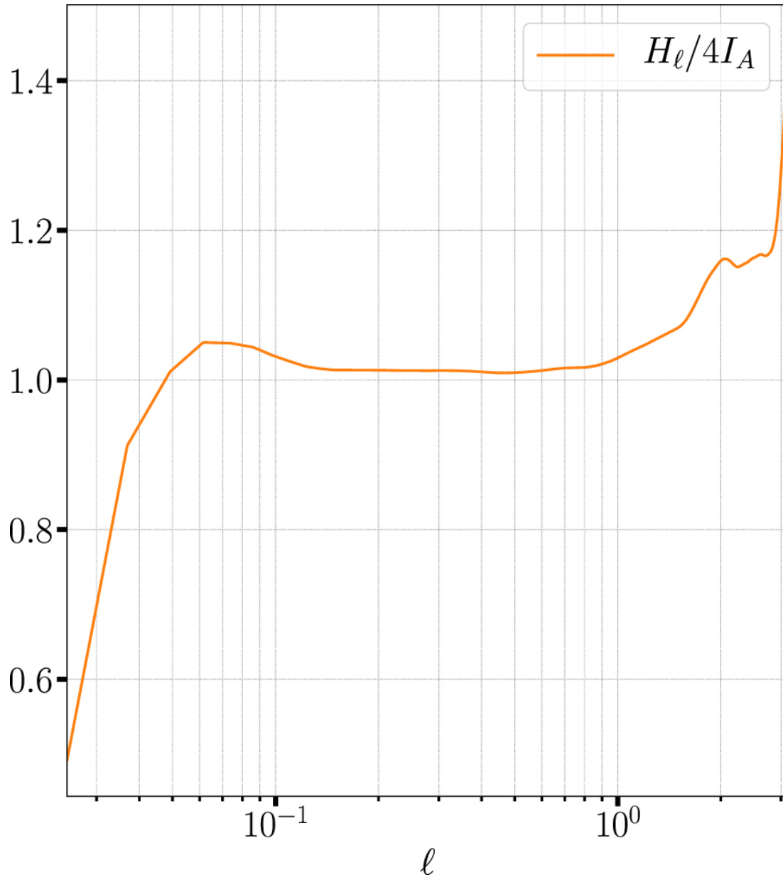
Figure 1. from On Exact Laws in Incompressible Hall Magnetohydrodynamic Turbulence null 2019 APJ 881 50 doi:10.3847/1538-4357/ab2be9 https://dx.doi.org/10.3847/1538-4357/ab2be9 © 2019. The American Astronomical Society. All rights reserved.
