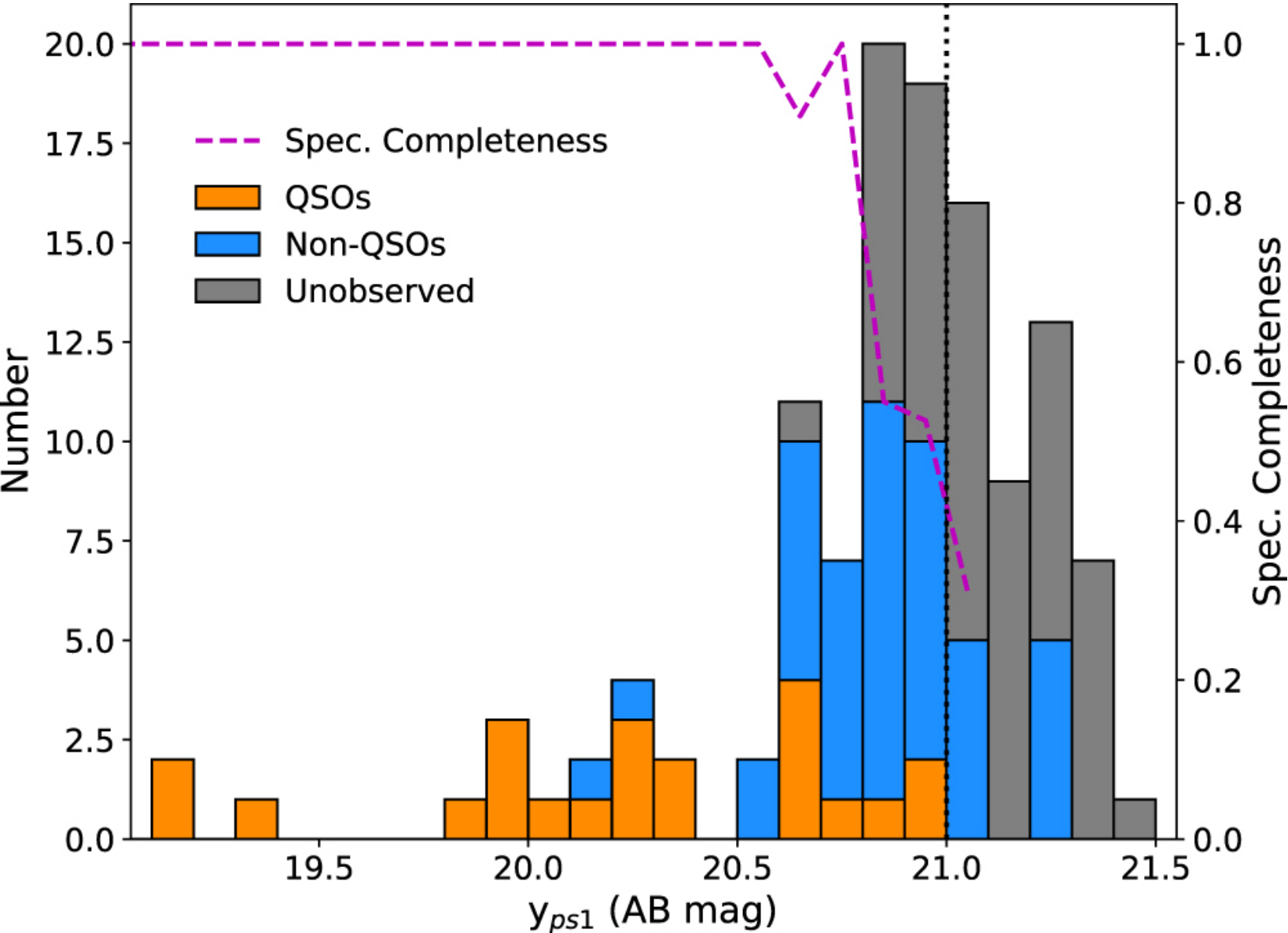
Figure 8. from Exploring Reionization-era Quasars. III. Discovery of 16 Quasars at 6.4 < z < 6.9 with DESI Legacy Imaging Surveys and the UKIRT Hemisphere Survey and Quasar Luminosity Function at z \sim 6.7 null 2019 APJ 884 30 doi:10.3847/1538-4357/ab2be5 https://dx.doi.org/10.3847/1538-4357/ab2be5 © 2019. The American Astronomical Society. All rights reserved.
