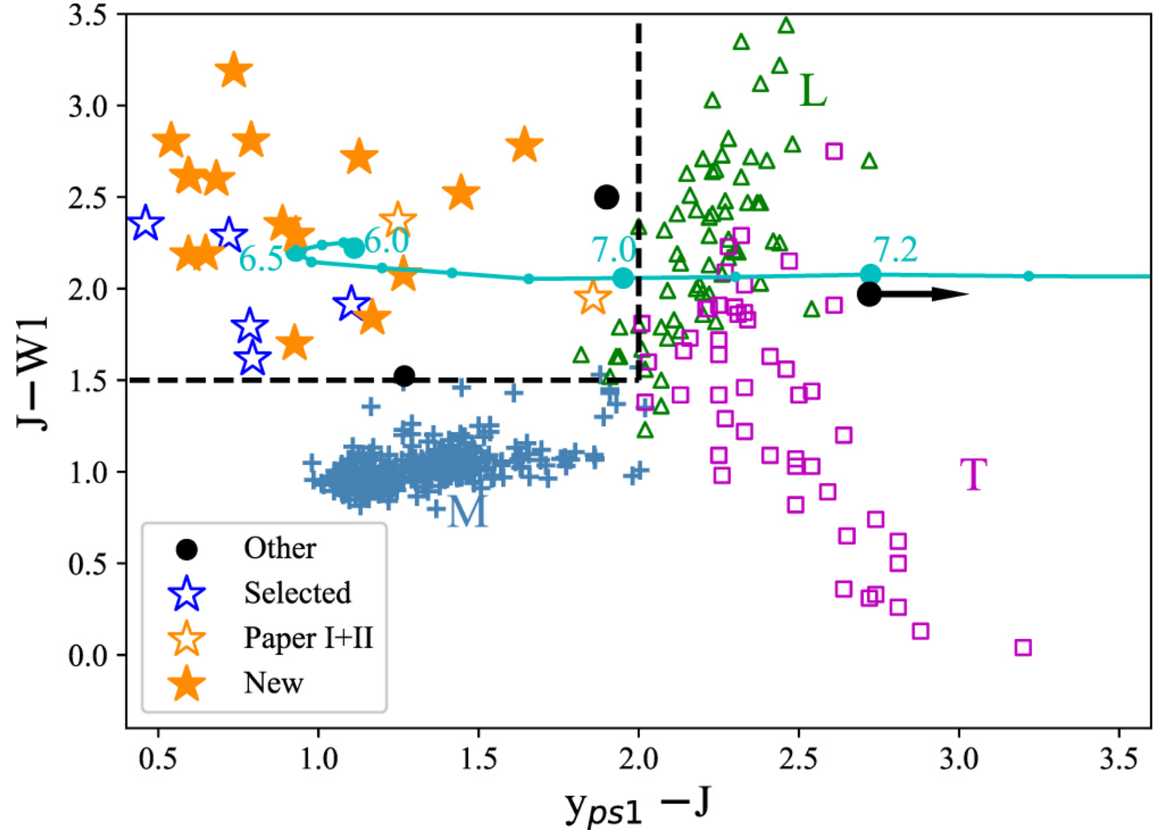
Figure 1. from Exploring Reionization-era Quasars. III. Discovery of 16 Quasars at 6.4 < z < 6.9 with DESI Legacy Imaging Surveys and the UKIRT Hemisphere Survey and Quasar Luminosity Function at z \sim 6.7 null 2019 APJ 884 30 doi:10.3847/1538-4357/ab2be5 https://dx.doi.org/10.3847/1538-4357/ab2be5 © 2019. The American Astronomical Society. All rights reserved.
