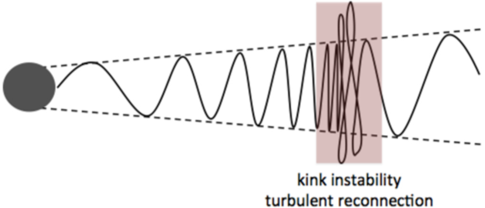
Figure 1. from Gamma-Ray Bursts Induced by Turbulent Reconnection null 2019 APJ 882 184 doi:10.3847/1538-4357/ab2b38 https://dx.doi.org/10.3847/1538-4357/ab2b38 © 2019. The American Astronomical Society. All rights reserved.
