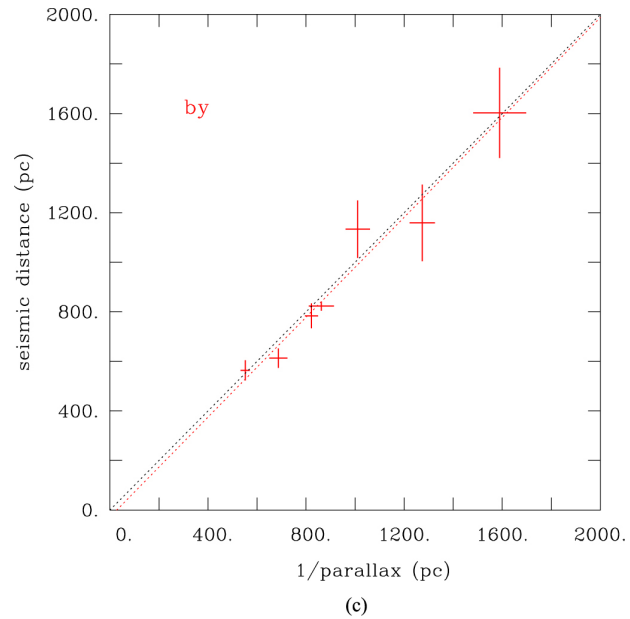
Figure 3. from Testing Seismic Models of Hot B Subdwarfs with Gaia Data null 2019 APJ 880 79 doi:10.3847/1538-4357/ab2885 https://dx.doi.org/10.3847/1538-4357/ab2885 © 2019. The American Astronomical Society. All rights reserved.
