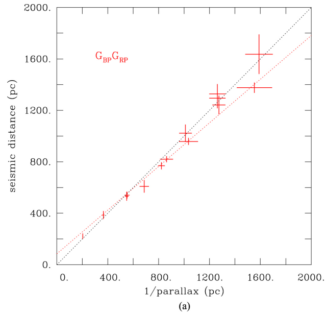
Figure 3. from Testing Seismic Models of Hot B Subdwarfs with Gaia Data null 2019 APJ 880 79 doi:10.3847/1538-4357/ab2885 https://dx.doi.org/10.3847/1538-4357/ab2885
