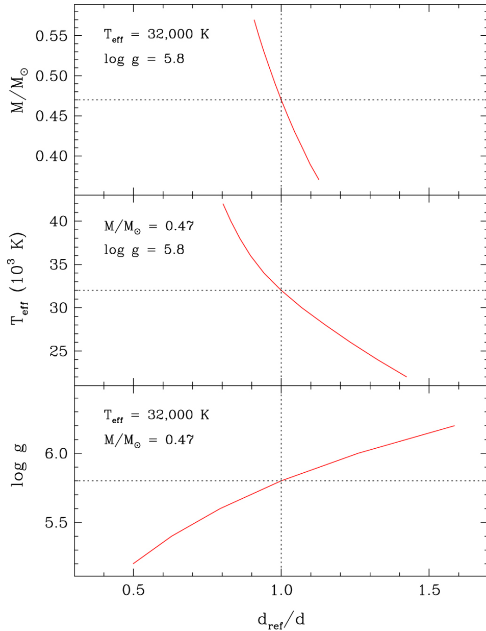
Figure 2. from Testing Seismic Models of Hot B Subdwarfs with Gaia Data null 2019 APJ 880 79 doi:10.3847/1538-4357/ab2885 https://dx.doi.org/10.3847/1538-4357/ab2885 © 2019. The American Astronomical Society. All rights reserved.
