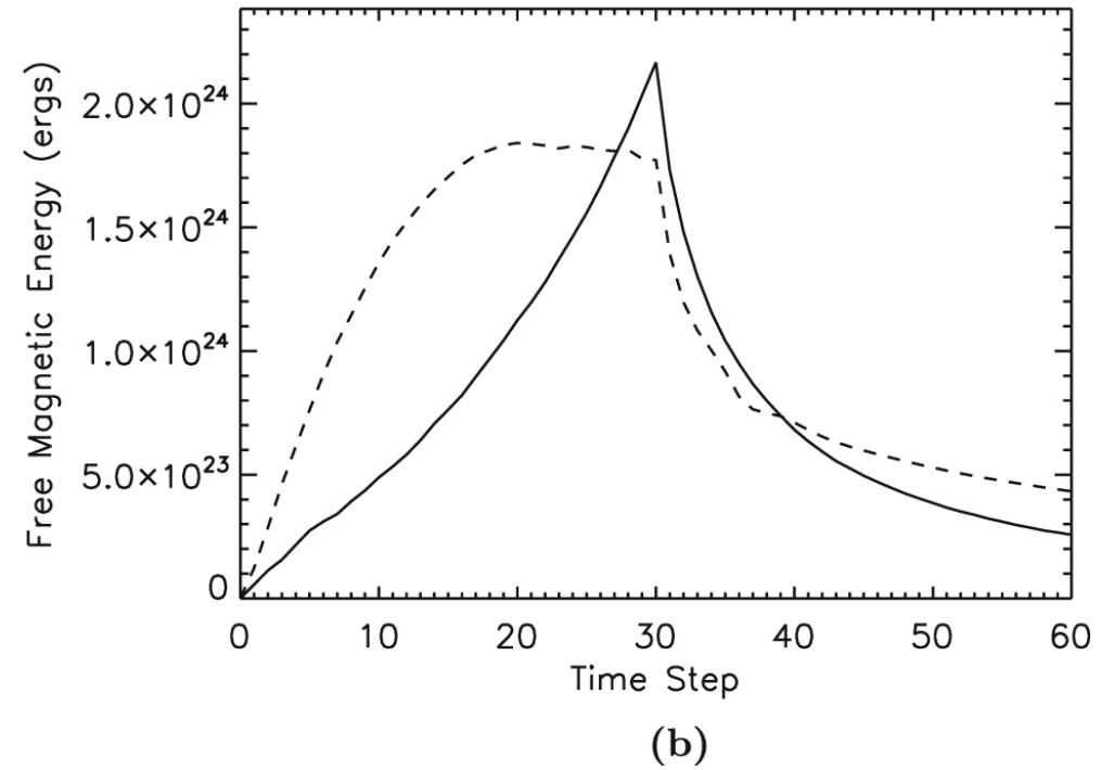
Figure 9. from Nonlinear Force-free Field Modeling of Solar Coronal Jets in Theoretical Configurations null 2019 APJ 880 62 doi:10.3847/1538-4357/ab271a https://dx.doi.org/10.3847/1538-4357/ab271a © 2019. The American Astronomical Society. All rights reserved.
