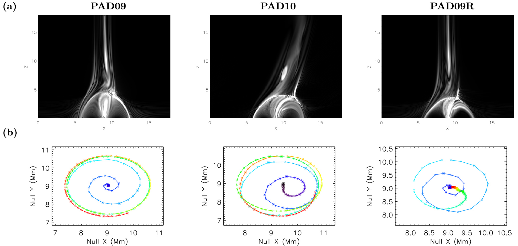
Figure 5. from Nonlinear Force-free Field Modeling of Solar Coronal Jets in Theoretical Configurations null 2019 APJ 880 62 doi:10.3847/1538-4357/ab271a https://dx.doi.org/10.3847/1538-4357/ab271a © 2019. The American Astronomical Society. All rights reserved.
